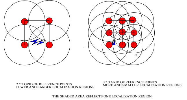
Fig. 1. Granularity of Localization Regions vs. Range Overlap
