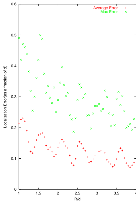
Fig. 6. Localization Error vs. Overlap, R/d . (Simulations)
